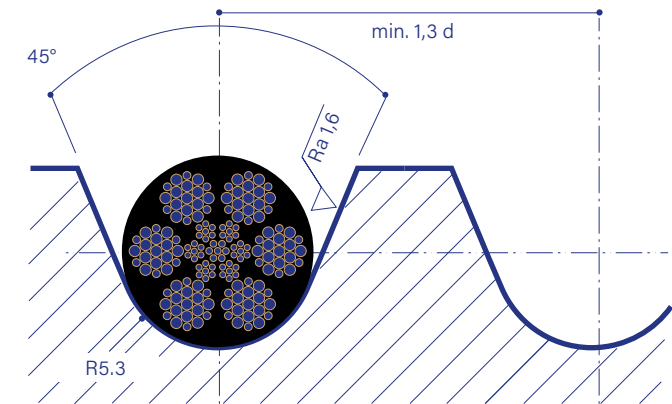
Specified Groove Diagram for CTP® 10 mm
