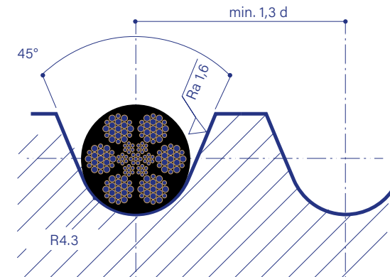
Specified Groove Diagram for CTP® 8.1 mm
