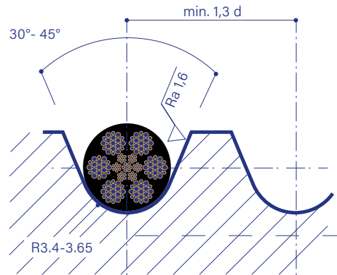
Specified Groove Diagram for CTP® 6.5 mm
